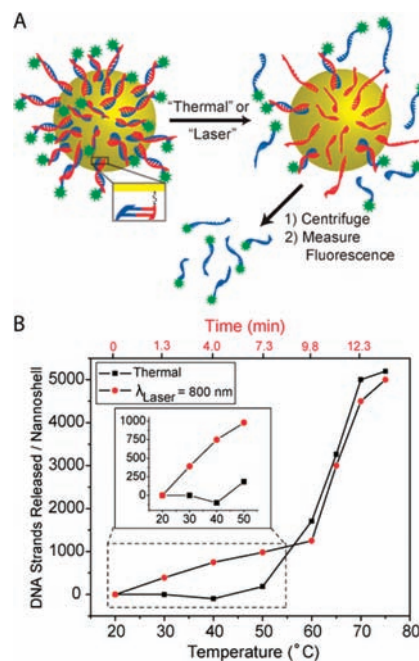
Figure 2. Thermal and light-triggered release of ssDNA from nanoshells. (A) Schematic of ssDNA release from gold nanoshells. The thiolated host sequence (red) attaches to the gold surface. The cargo complementary sequence (blue) is tagged with a fluorescein molecule (green). Upon heating (thermal treatment) or illumination with laser light (laser treatment) the fluorescein-tagged sequence is released and subsequently separated from the nanoshells by centrifugation. The fluorescence is then measured and normalized by nanoshell concentration. (B) Number of DNA strands released per nanoshell as a function of solution temperature for thermal treatment (black squares) and laser treatment (red dots). Inset shows the expanded view of the temperature range prior to thermal melting where light-triggered release is observed.
