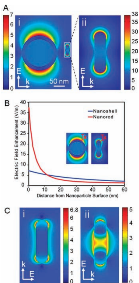
Figure 4. Near-field intensity enhancements of nanoshells ( [r_1, r_2] = [60, 76] nm) and nanorods ( [w, l] = [13, 47] nm) calculated using the finite-element method (FEM). (A) Enhancements for a (i) nanoshell and (ii) nanorod (longitudinal polarization) when driven at \lambda = 800 nm. Inset of nanorod depicts the size difference between nanoshells and nanorods. (B) Electric field enhancement as a function of distance from the nanoparticle surface in the polarization direction for nanoshells (blue) and nanorods (red). (C) Nanorod enhancements when driven at \lambda = 532 nm for: (i) transverse polarization and (ii) longitudinal polarization.
