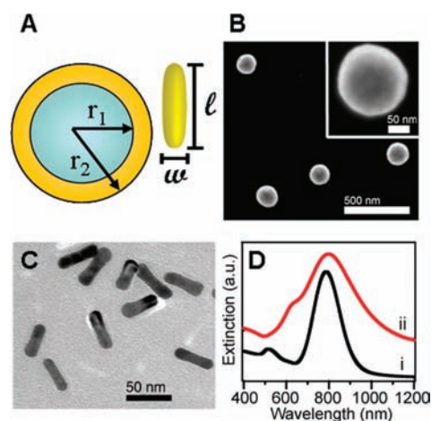
Figure 1. (A) Schematic of nanoshells ( [r_1, r_2] = [60, 76] nm) and nanorods ( [w, l] = [13, 47] nm) used in this series of experiments. (B) SEM image of nanoshells and (C) TEM image of nanorods. (D) Extinction spectra of solution of (i) nanorods with ( \lambda_{\max} \approx 788 nm) and (ii) nanoshells with ( \lambda_{\max} \approx 797 nm). Spectra are slightly vertically offset for clarity.
